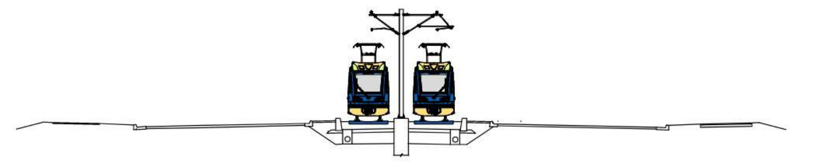
TYPICAL SECTION AT GRADE
