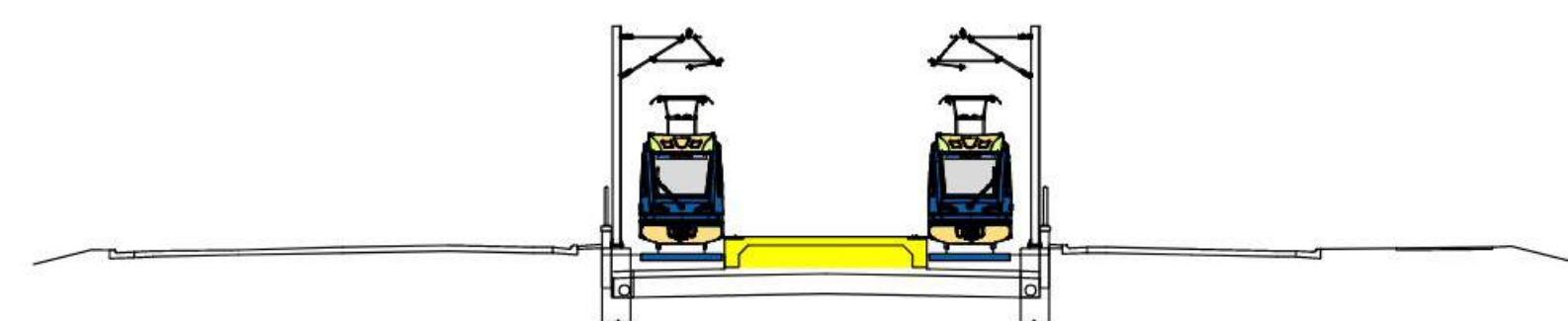
TYPICAL SECTION AT STATION
