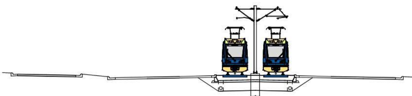
TYPICAL SECTION
