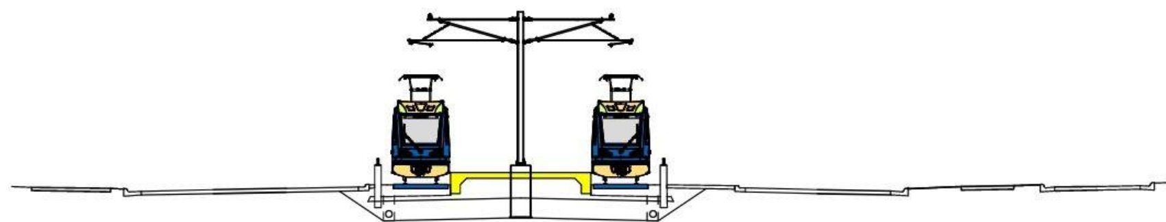
TYPICAL SECTION AT STATION
